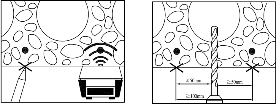
Drawing B4. Installation process in prestressed hollow core concrete slabs
