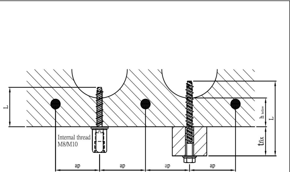
Drawing A4. Installed condition in prestressed hollow core concrete slabs
