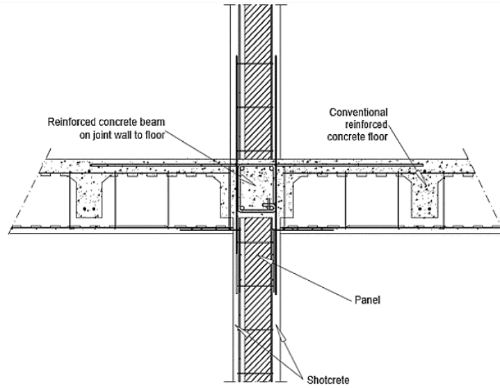
Figure A1.3. Schematic example of GREEN WALLS BUILDING SYSTEM internal wall-floor joining.
