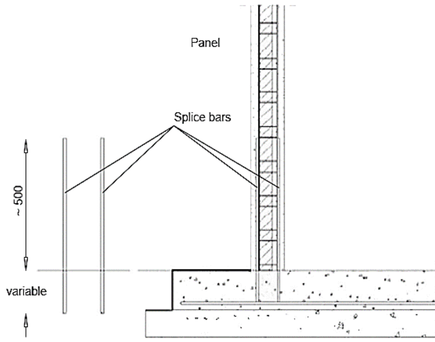
Figure A3.1. Joint wall to sub-structure – vertical section – example
