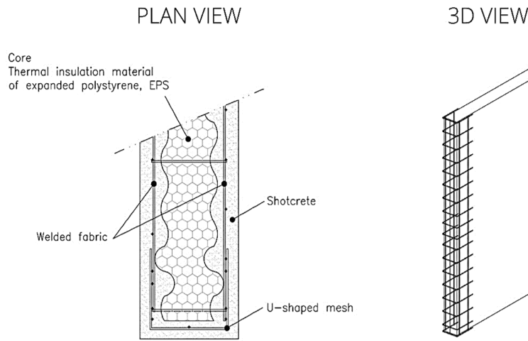
Figure A2.3. Use of U-shaped meshes. Example.
