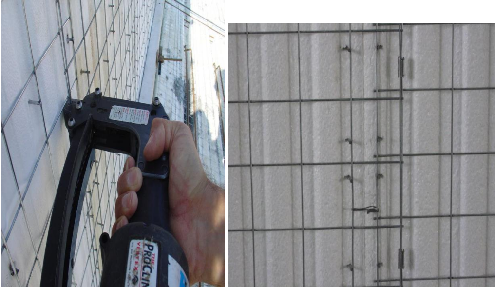
Figure A3. 3. Tying continuous panels with staplers / clamps. Example.
