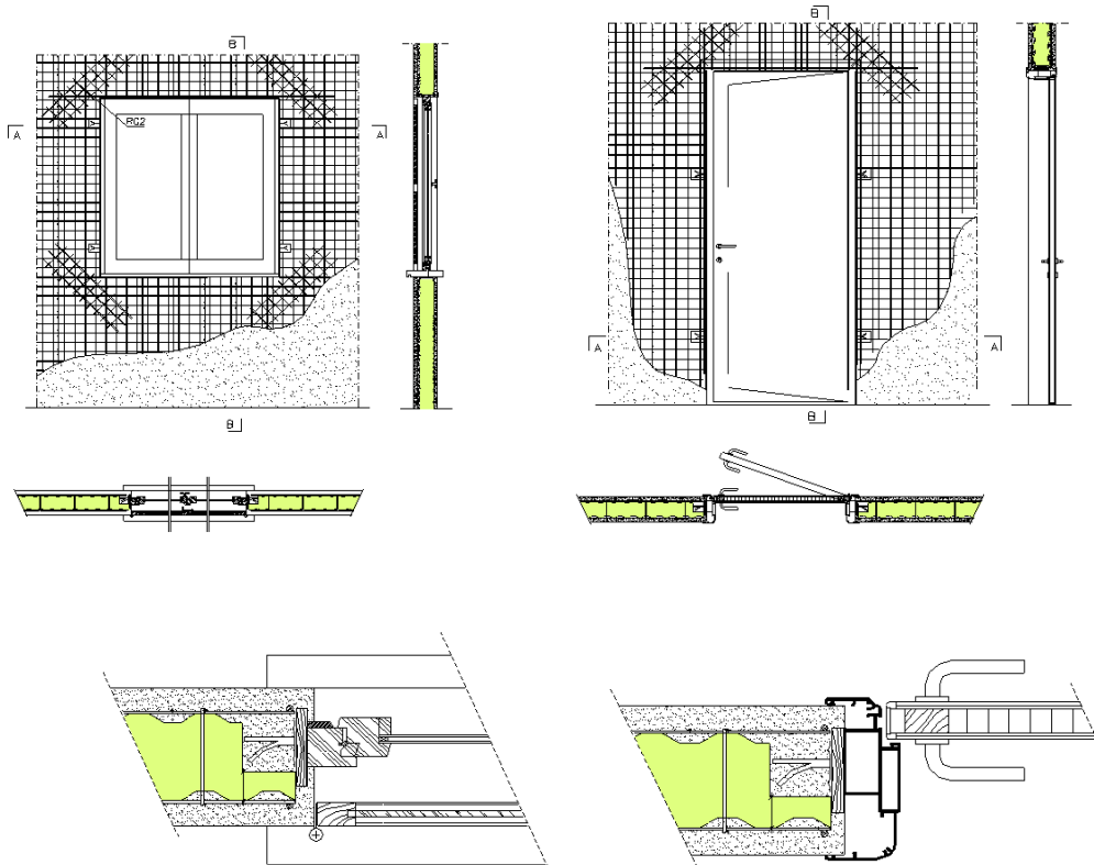
Figure A2.2. Use of flat reinforcing meshes (vertical and horizontal sections). Example.
