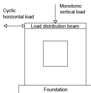
Figure B2.3. Type 3: dimensions 300 x 300 x 15 cm (aspect ratio 1:1), window opening (1.0 x 1.0 m) in the centre of the panel.
