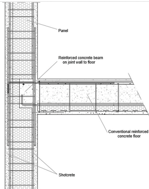
Figure A1.2. Schematic example of GREEN WALLS BUILDING SYSTEM external wall-floor joining
