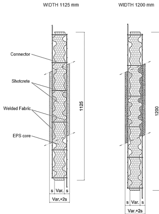
Figure A1.4. Cross section of the installed panel, dimensions in mm.
