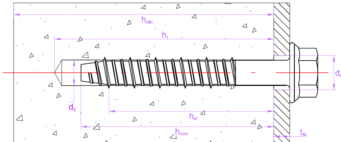
Drawing B1. Installed condition for anchors CS-W and CS-C.
