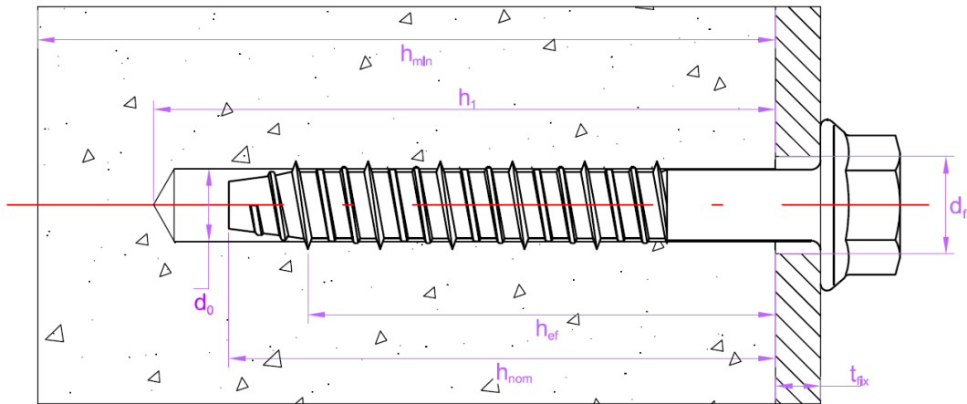
Drawing A1. Installed condition for anchors CS-W and CS-C.
