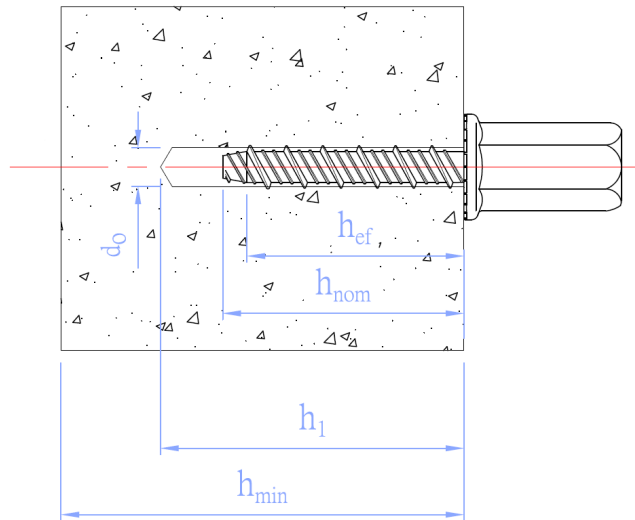
Drawing A2. Installed condition for anchors AMDTH, AMROD, AMROF, AMROH, AMRHH, AMROO, AMRCC, AMRHC and AMROC
