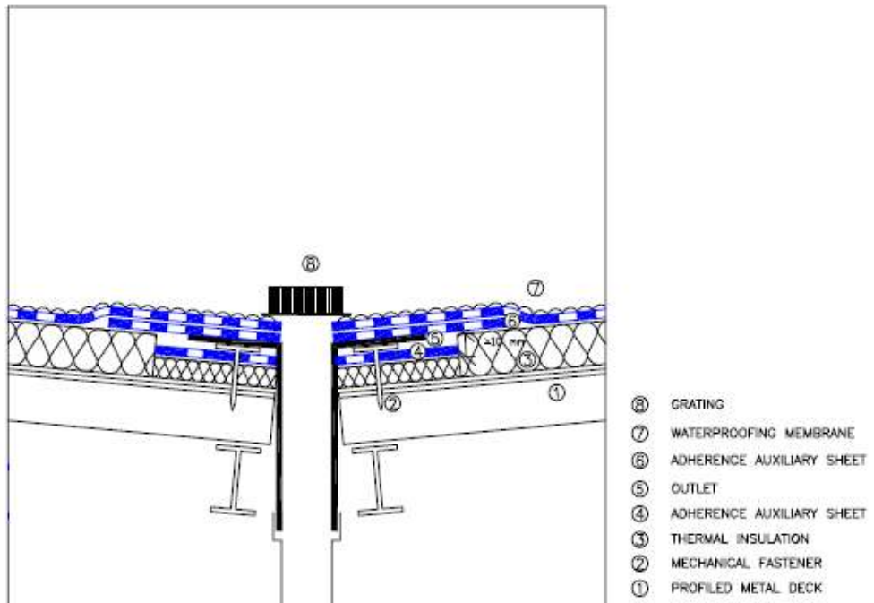
Fig. 4 Drain detail
